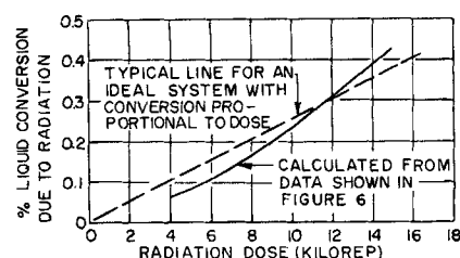
Fig. 7. Radiation conversion (total liquid conversion minus thermal) vs. dose.
