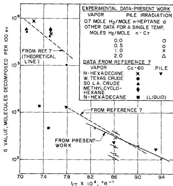
Fig. 4. A comparison of G values obtained with other data from the literature.
